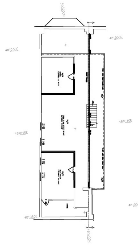
First Floor Plan - Scale 1-100@A1
